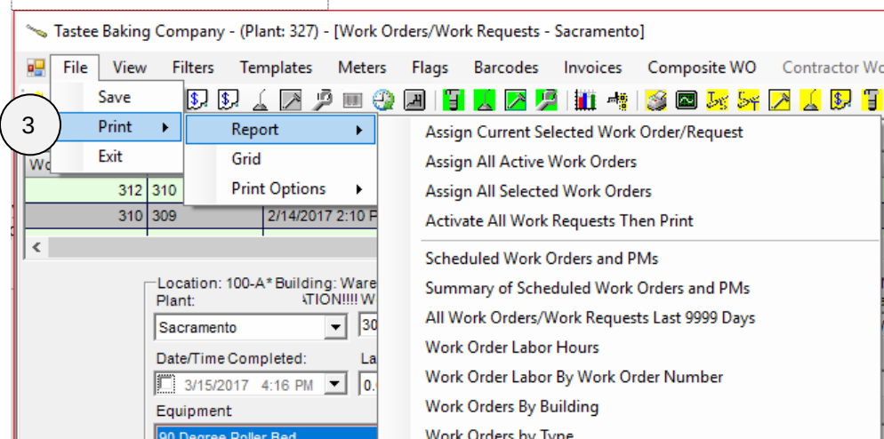
FIGURE 4.3 – PRINT REPORTS
