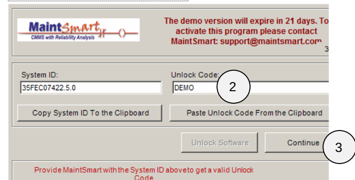
FIGURE 1.2 – LICENSE SCREEN
